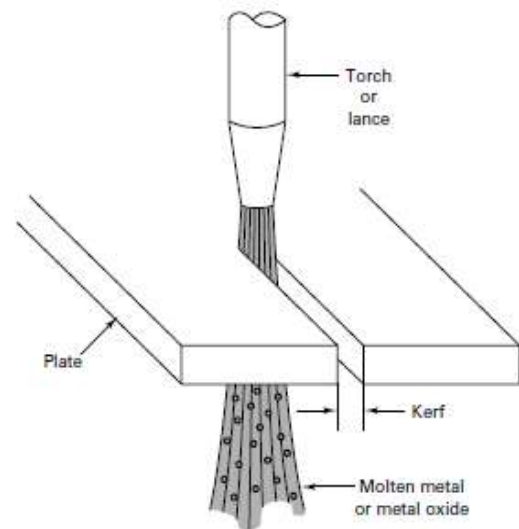
Figure 3: Gas cutting of a metal plate
