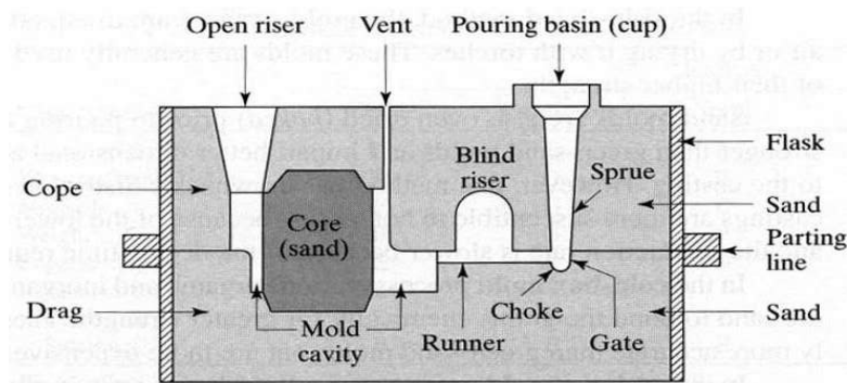
Figure 1: Gating System
